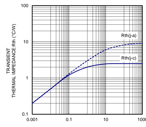
R_th-t CHARACTERISTICS
