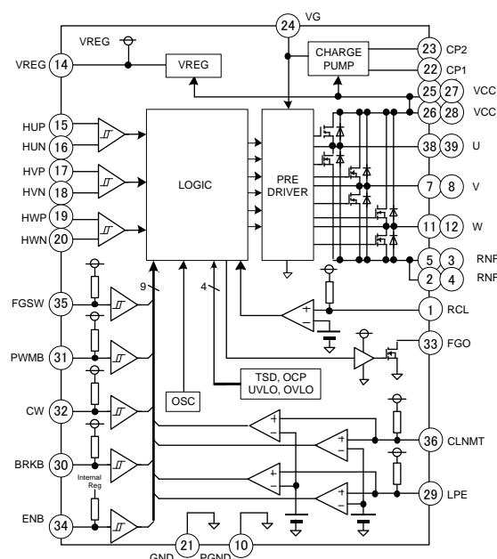
Figure 3. Block Diagram
