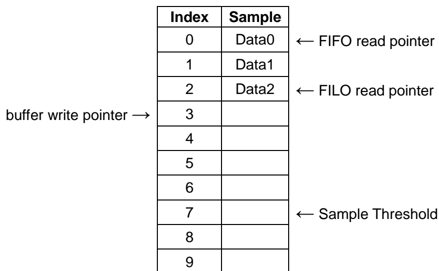
Figure 17: Buffer Filling
