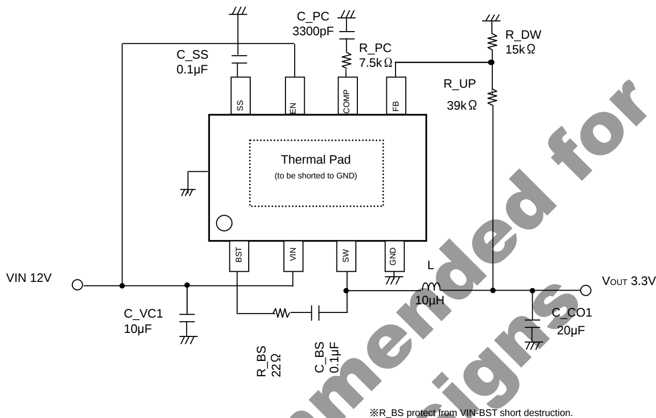
Fig.18 Application Circuit
