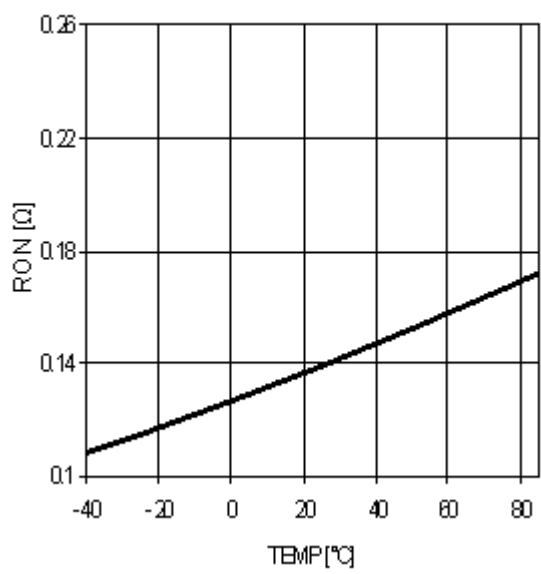
Fig.8 Hi,Low-Side On-resistance
