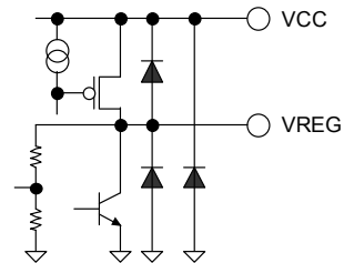
Figure 37. VREG, VCC
