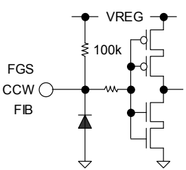
Figure 40. FGS, CCW, FIB
