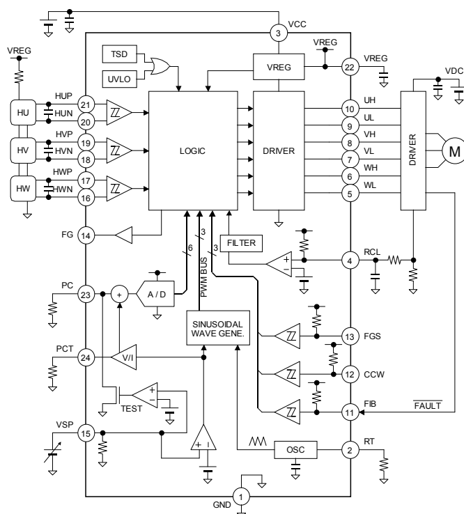
Figure 2. Block diagram
