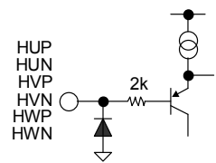
Figure 39. HXP, HXN
