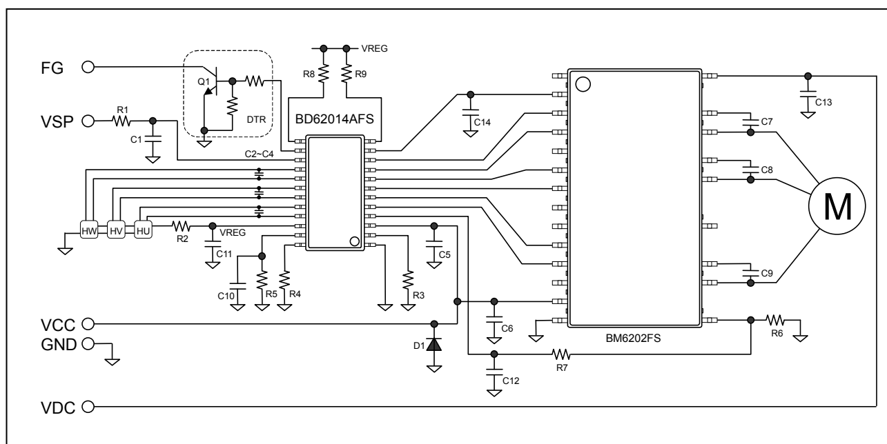
Figure 1. Application circuit example - BD62014AFS &amp; BM6202FS
