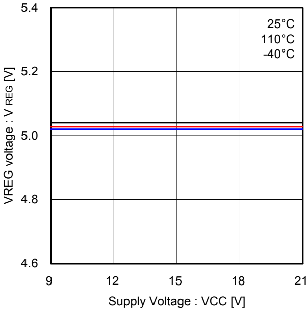
Figure 10. VREG - VCC
