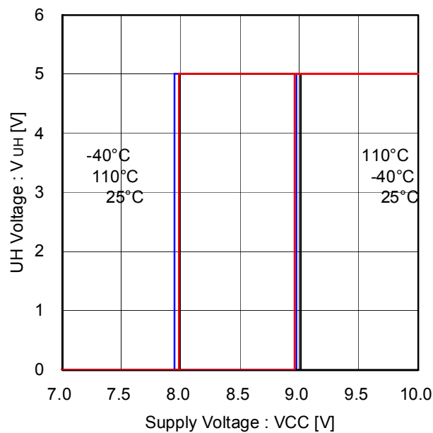
Figure 28. Under voltage lock out (VCC)
