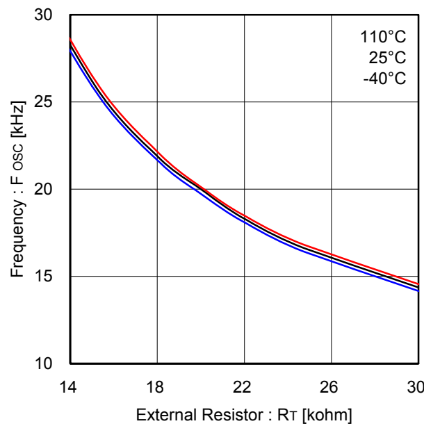
Figure 32. Carrier frequency - R_T
