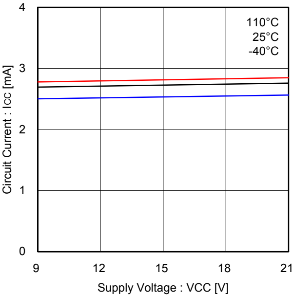
Figure 9. Circuit current
