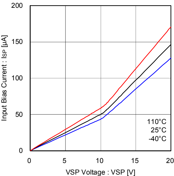
Figure 16. VSP input bias current
