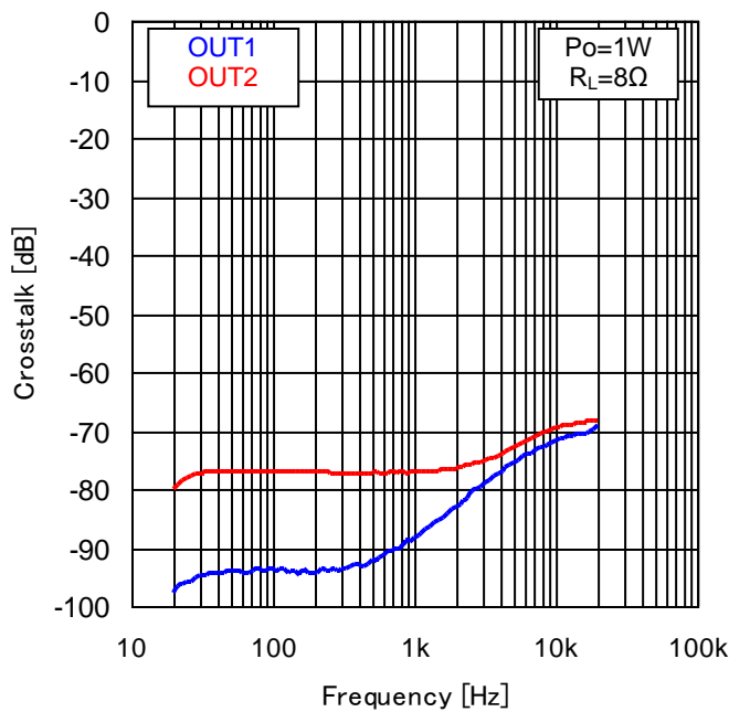
Figure 20. Frequency - Crosstalk
