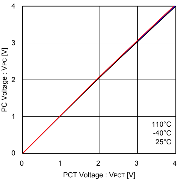
Figure 30. PCT - PC linearity (R PCT =R PC =100kΩ)
