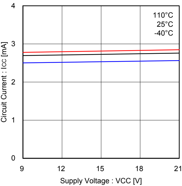
Figure 9. Circuit current
