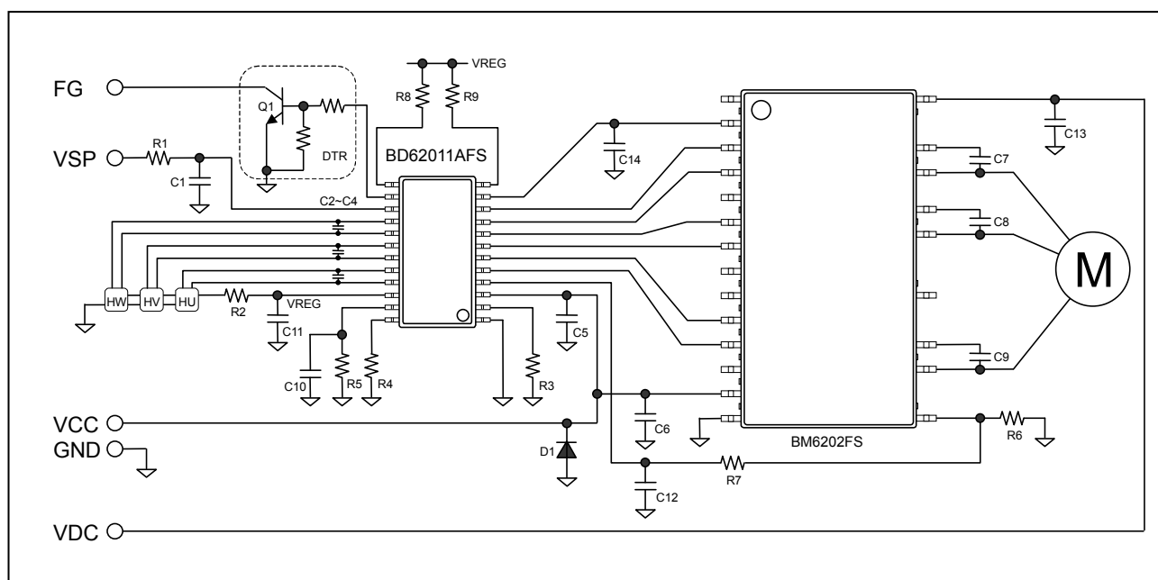
Figure 1. Application circuit example - BD62011AFS &amp; BM6202FS
