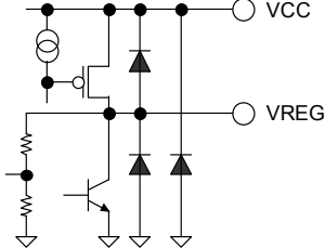
Figure 37. VREG, VCC
