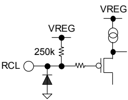
Figure 35. RCL
