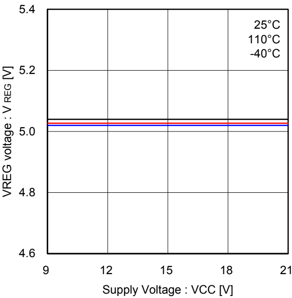
Figure 10. VREG - VCC
