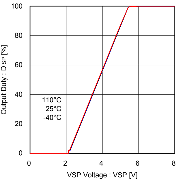
Figure 17. Output duty - VSP voltage
