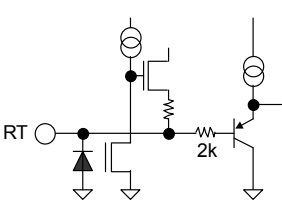
Figure 34. RT
