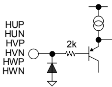
Figure 39. HXP, HXN
