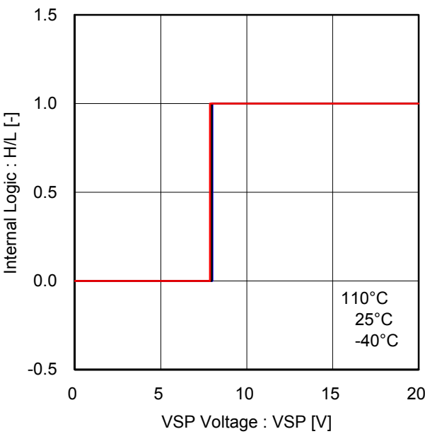
Figure 18. Testing mode threshold voltage
