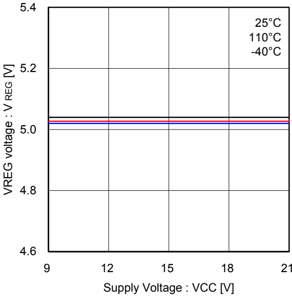
Figure 10. VREG - VCC
