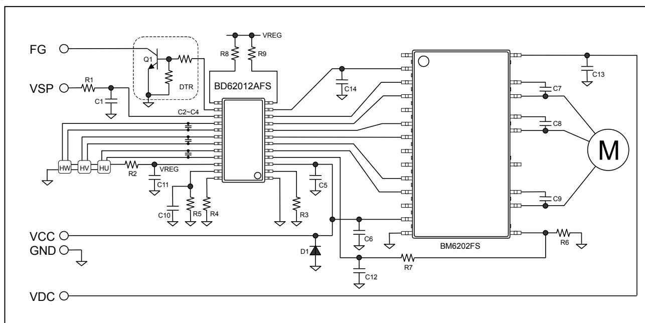
Figure 1. Application circuit example - BD62012AFS &amp; BM6202FS
