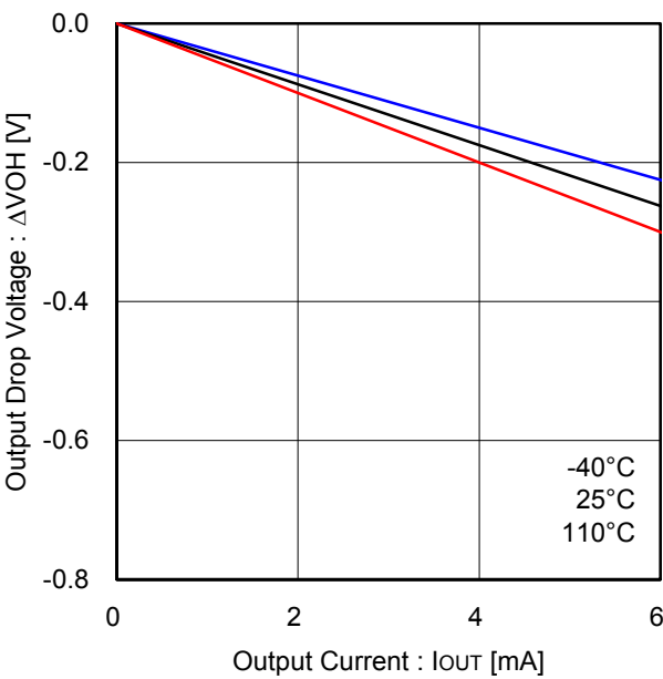
Figure 19. High side output voltage (FG)
