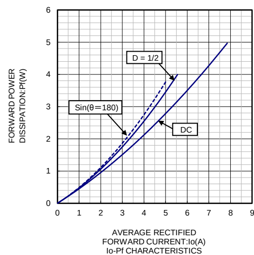
I_0 - P_F CHARACTERISTICS
