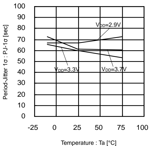
Figure 28. Period-Jitter 1 \sigma vs Temperature (36.9MHz)
