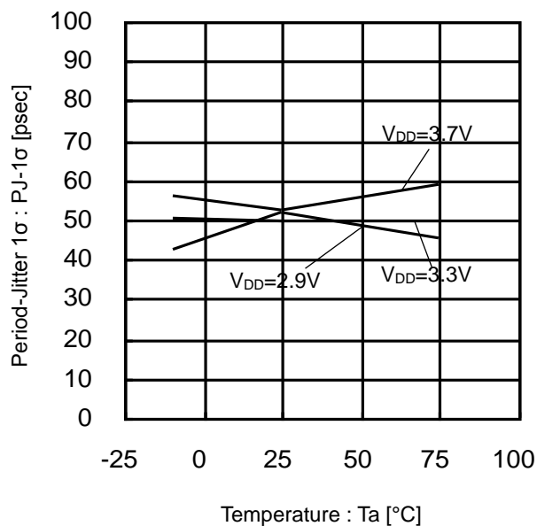
Figure 40. Period-Jitter 1σ vs Temperature (18.4MHz)
