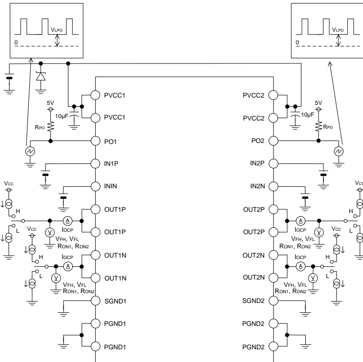
Figure 41. Measurement Circuit 2
