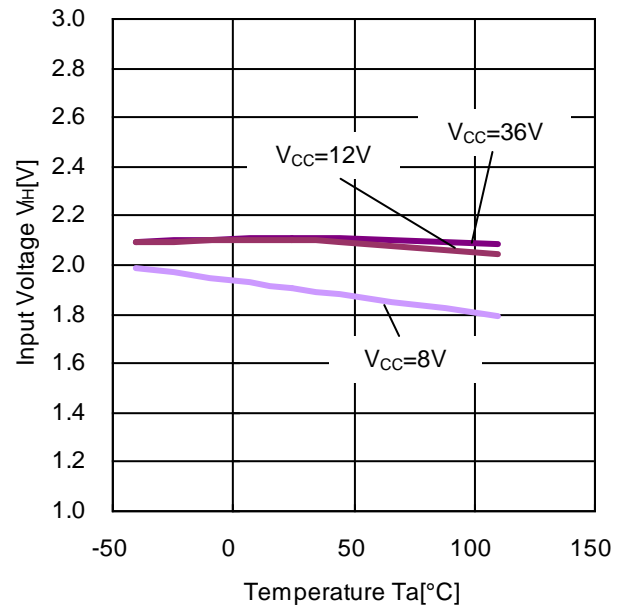
Figure 12. Input Voltage vs Temperature (Input H Voltage V_{IH} , V_{IN}=0V \rightarrow 5.0V )
