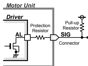
Figure 58. Protection of AL Terminal
