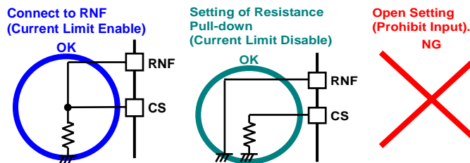
Figure 45. CS Terminal Setting
