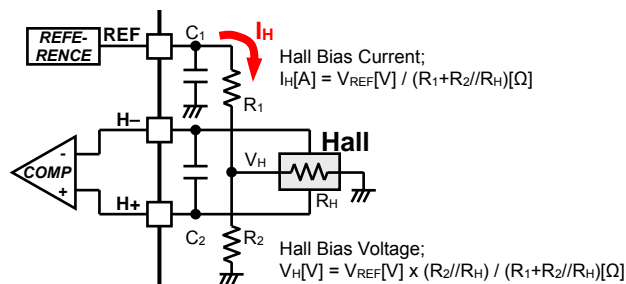
Figure 53. Hall Input Application
