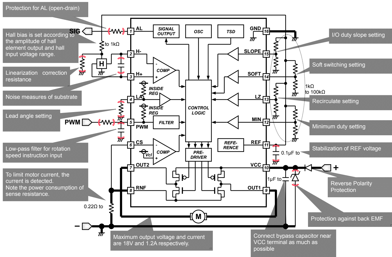
Figure 23. PWM Input Application
