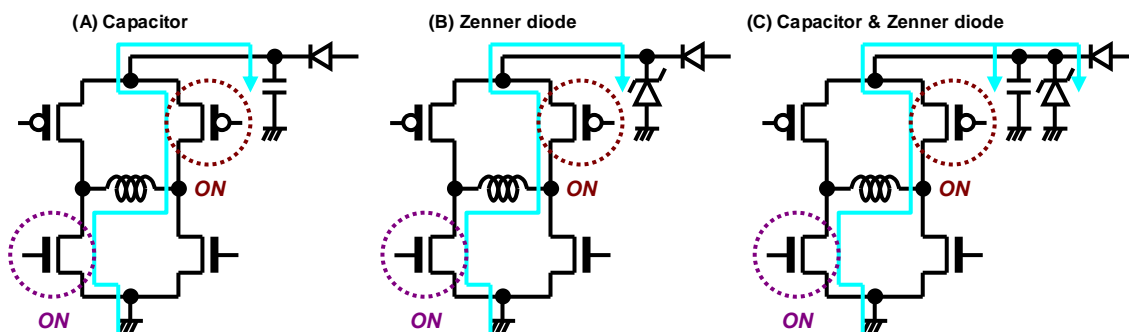
Figure 56. Measure against V CC and Motor Driving Outputs Voltage
