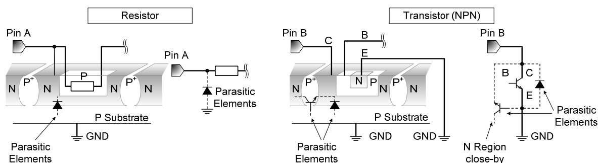
Figure 62. Example of Monolithic IC Structure
