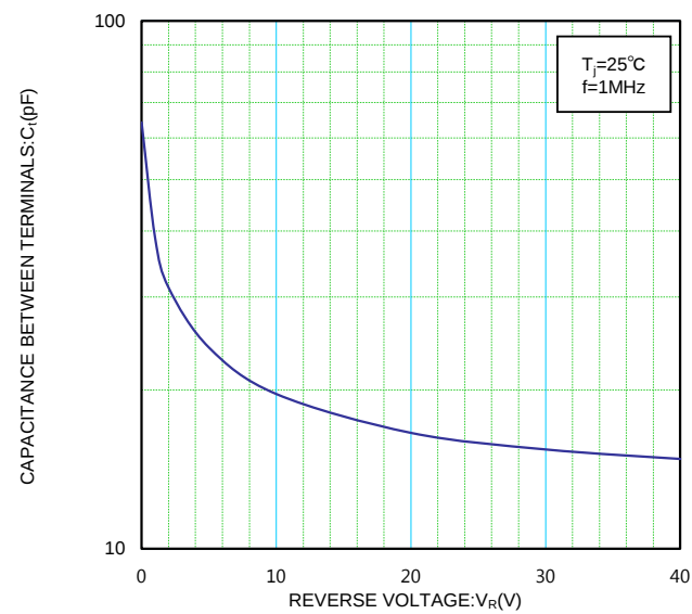
V R -C t CHARACTERISTICS
