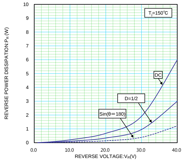
V_R - P_R CHARACTERISTICS
