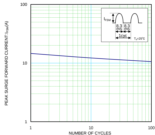
I FSM -CYCLE CHARACTERISTICS
