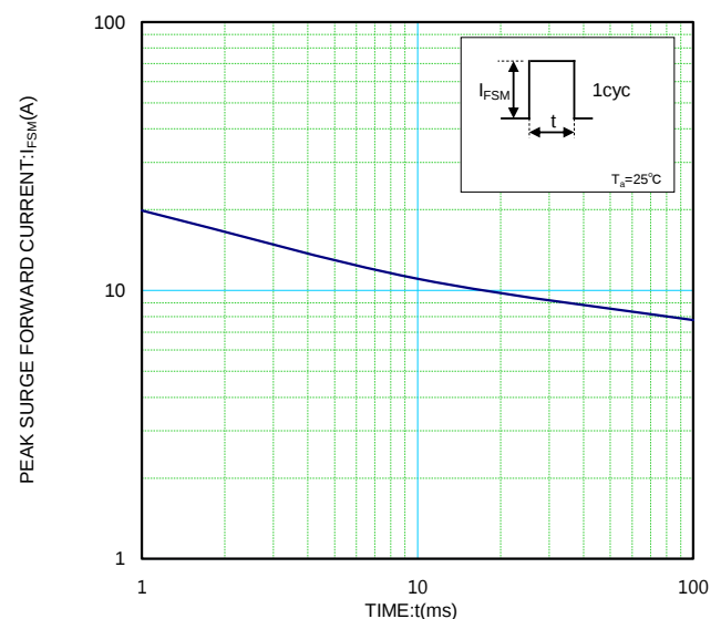
I FSM -t CHARACTERISTICS
