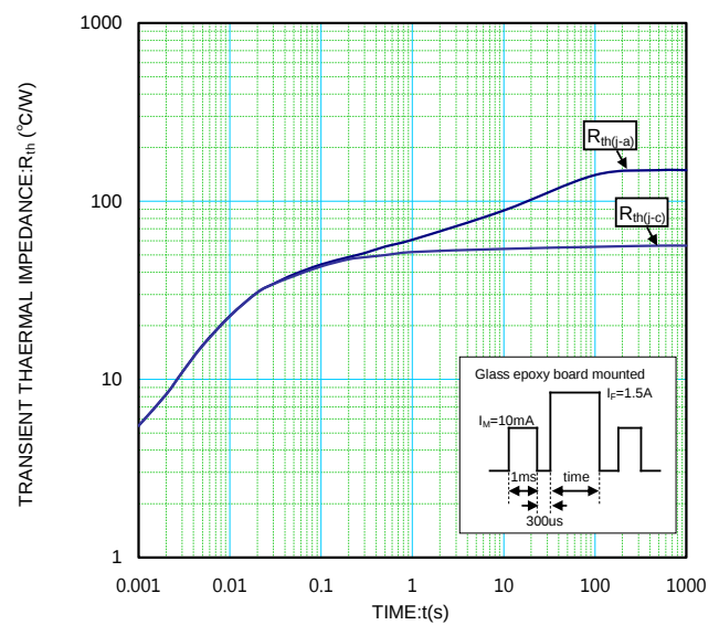
R th -t CHARACTERISTICS
