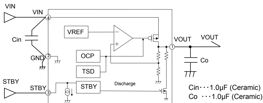
Figure 2. Block Diagrams
