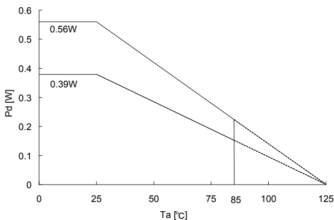
Figure 103. SSON004X1010 Power dissipation heat reduction characteristics (Reference)
