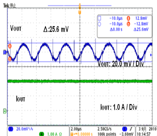
Figure 16. Output Ripple Voltage (V_{\text{IN}} = 12 \text{ V } V_{\text{OUT}} = 3.3 \text{ V } L = 10 \mu\text{H } C_{\text{OUT}} = 20 \mu\text{F } I_{\text{OUT}} = 2.0 \text{ A})
