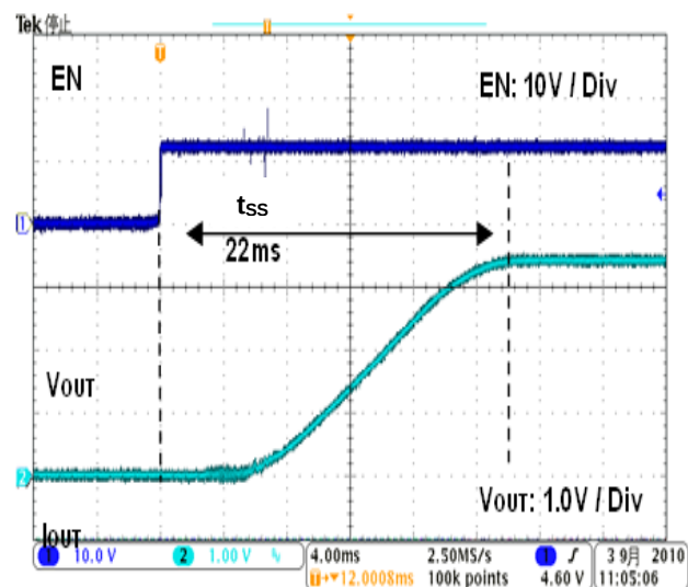
Figure 17. Start-Up Waveform (V_{\text{IN}} = 12 \text{ V } V_{\text{OUT}} = 3.3 \text{ V } L = 10 \mu\text{H } C_{\text{SS}} = 0.1 \mu\text{F})
