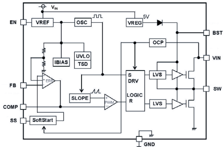
Figure 3. Block Diagram
