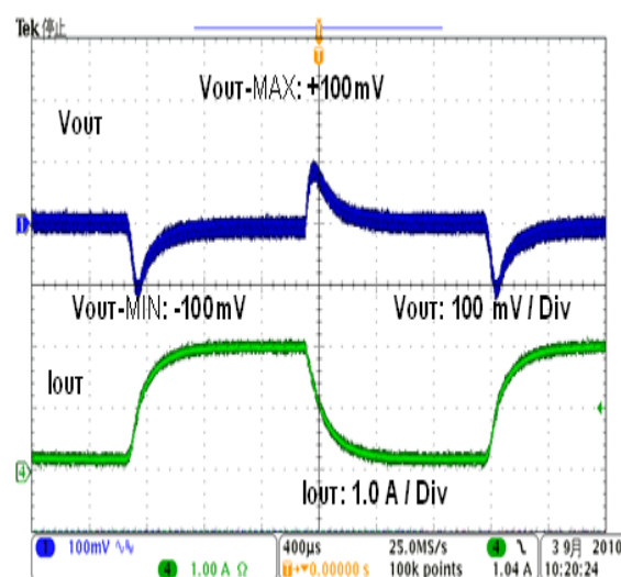
Figure 15. Transient Response ( V_{IN} = 12V V_{OUT} = 3.3V L = 10 \mu H C_{OUT} = 20 \mu F I_{OUT} = 0.2-2.0A)
