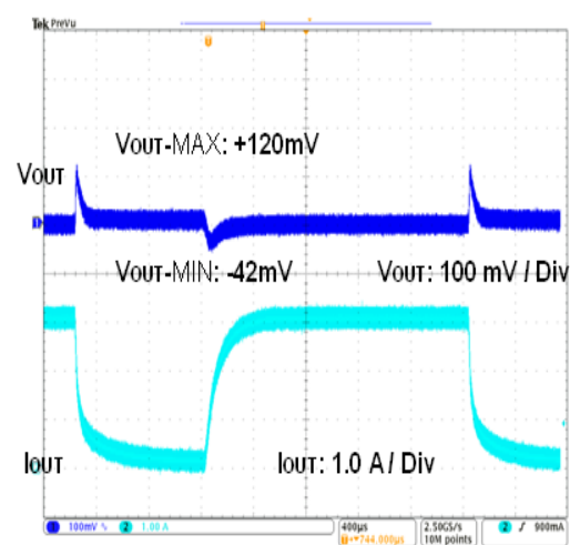
Figure 15. Transient Response ( V_{IN}=12V , V_{OUT}=3.3V , L=10\mu H , C_{OUT}=22\mu F , I_{OUT}=0.2A-3.0A )
