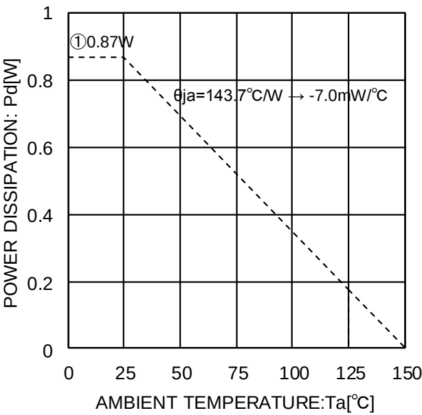
Figure 26. SSOP-B16 Power dissipation heat attenuation characteristics
