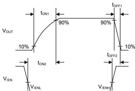
Figure 2. Timing Diagram(BD2045AFJ)
