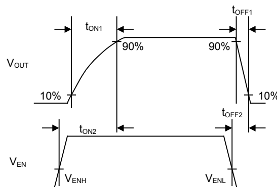
Figure 3. Timing Diagram (BD2055AFJ)
