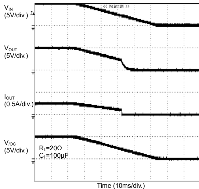
Figure 37. UVLO Response Decreasing V_{IN} (BD2045AFJ)
