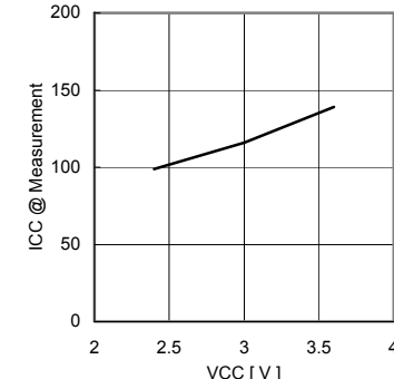
Fig.9 VCC - ICC (During measurement)
