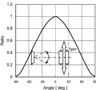
Fig.5 Directional Characteristics 2
