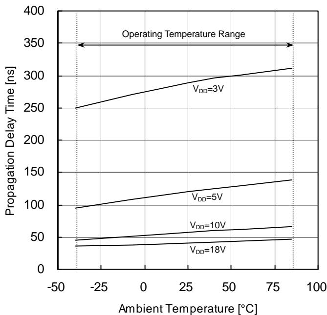
Figure 9. "H" to "L" Propagation delay time t_{PL}
