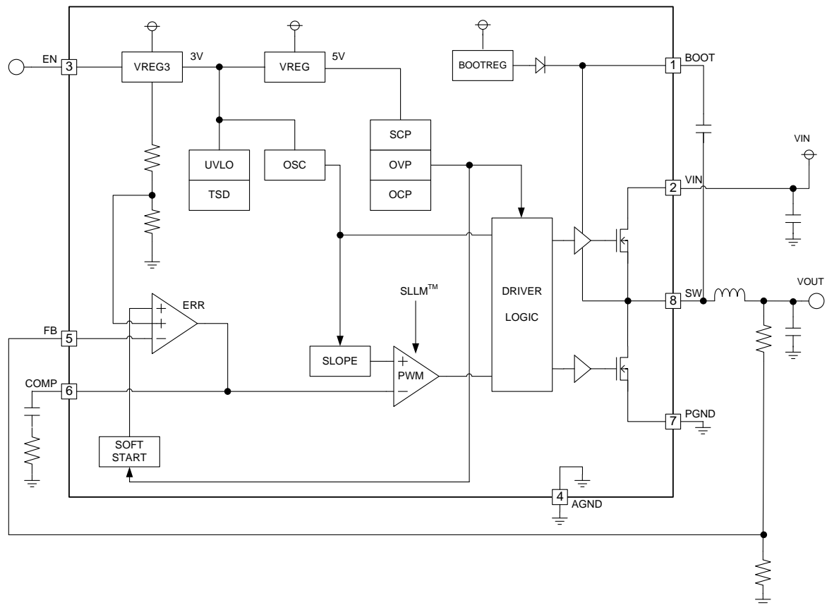
Figure 3. Block diagram
