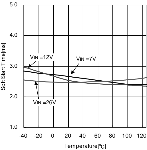
Figure 17. Soft Start Time - Temperature
