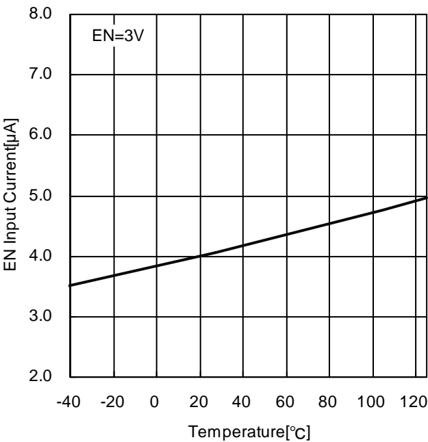
Figure 16. EN Input Current - Temperature
