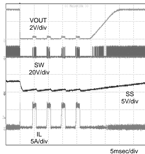
Figure 15. OCP function ( V_{\text{IN}}=12\text{V} , V_{\text{OUT}}=3.3\text{V} , L=4.7\mu\text{H} , C_{\text{OUT}}=20\mu\text{F} ) (VOUT is shorted to GND)
