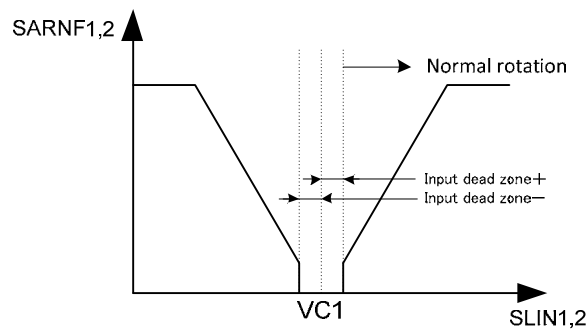
Figure 4. SLED Input vs Output Current
