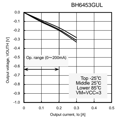
Fig.15 PMOS Output Voltage (BH6453GUL)
