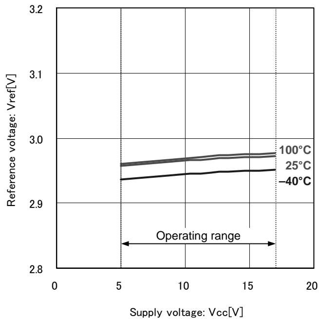
Fig.20 Reference voltage
