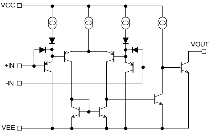
Fig.87 Circuit Diagram (one channel only )
