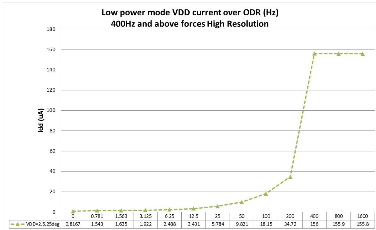
Figure 2: Current Profile
