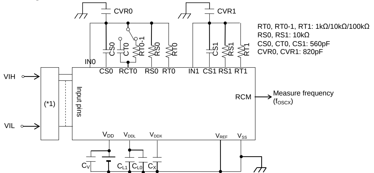
Measuring circuit
