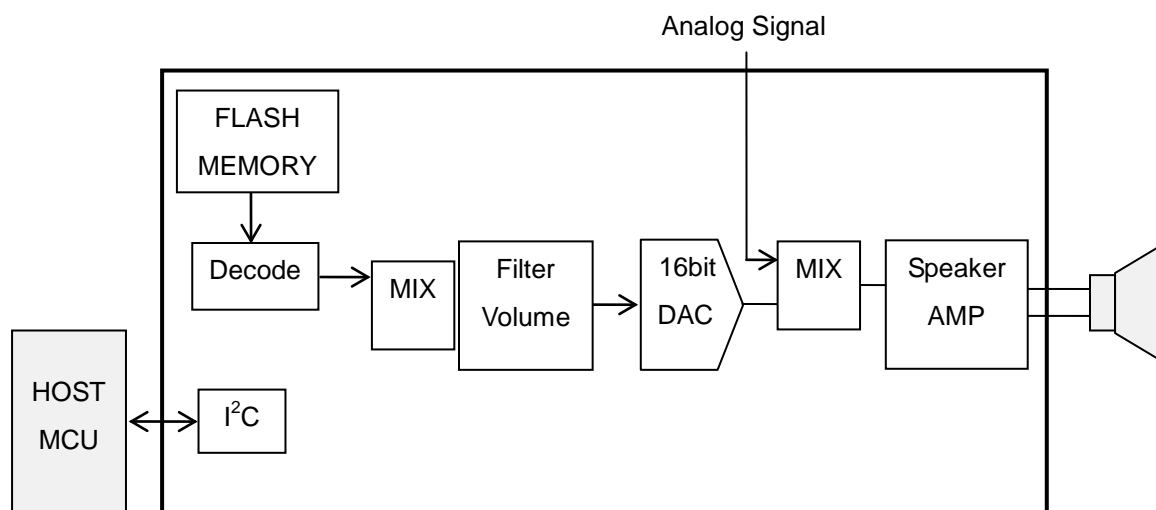
Application Circuit
