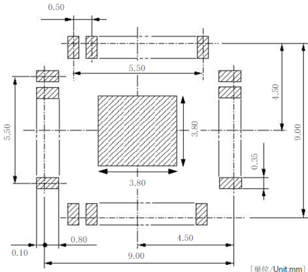
Mounting area for package lead soldering to PC boards
