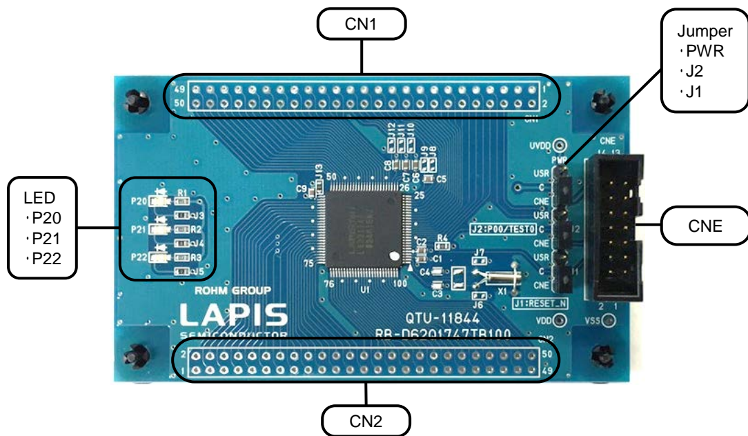
Fig. 1 ML62Q1747 Reference Board Outline Diagram
