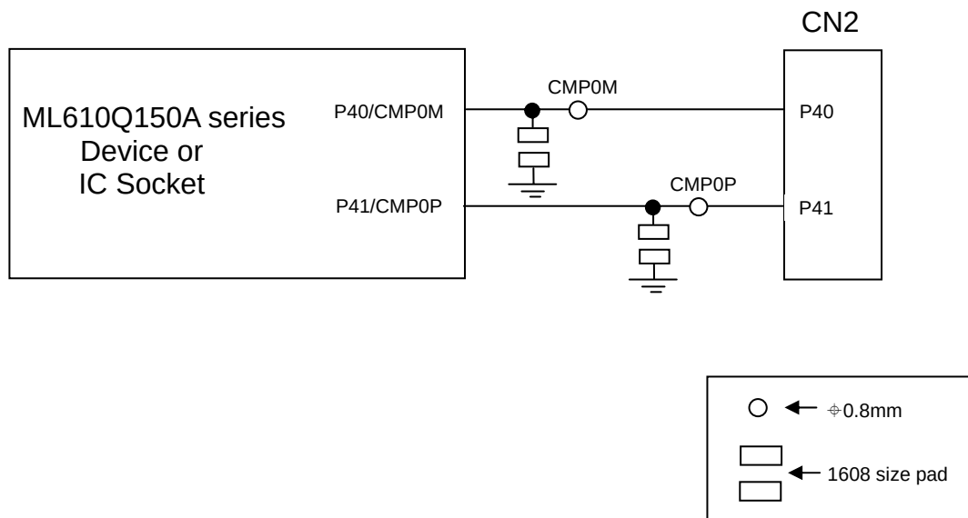
Fig.7 Analog Comparator Input
