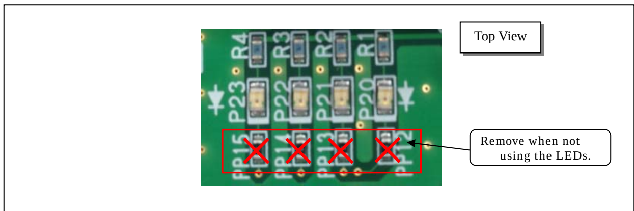
Fig.10 Zero-ohm resistors for LEDs
