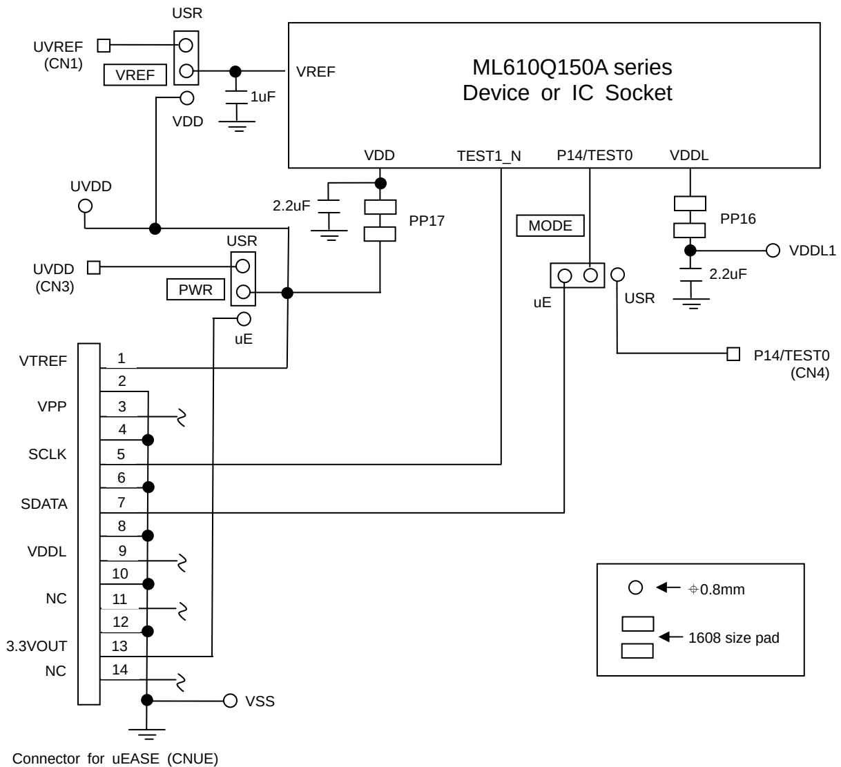
Fig.4 Power Circuit
