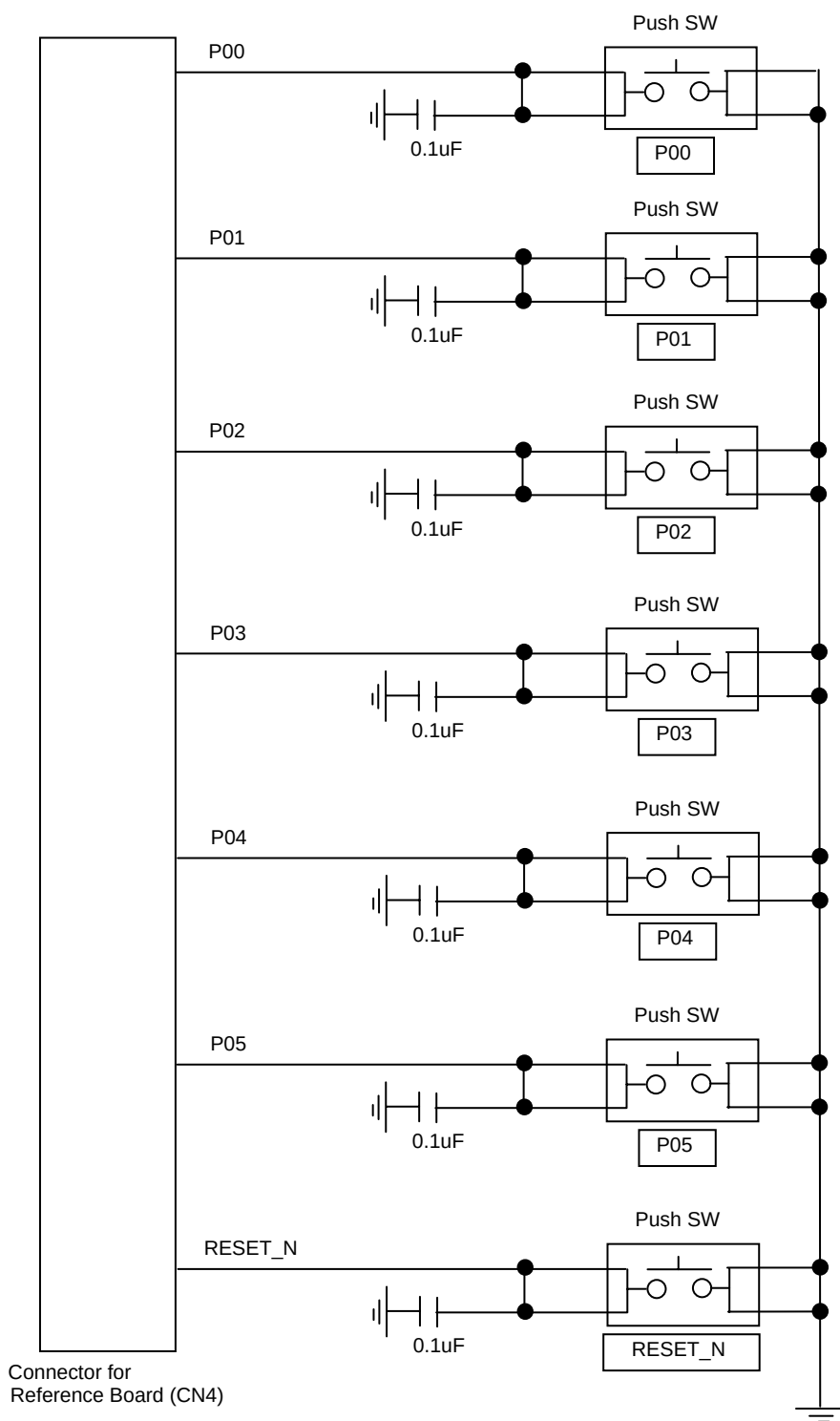
Fig.12 Input Switches
