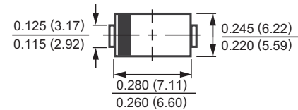
DO-214AB
