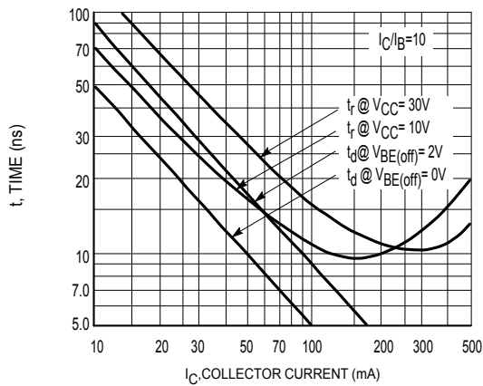
Figure 3. Turn-On Time
