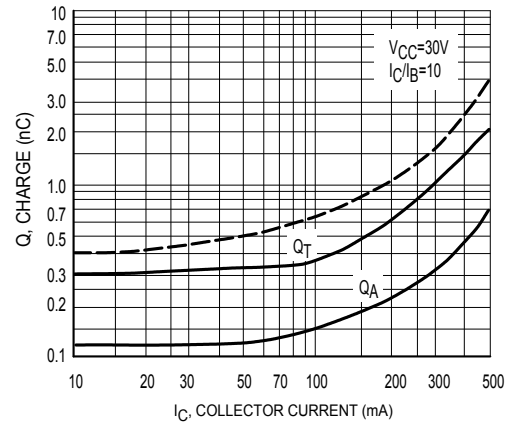
Figure 2. Charge Data
