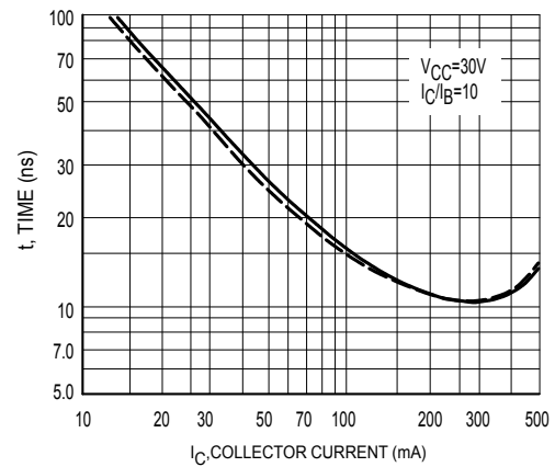
Figure 4. Rise Times
