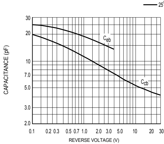
Figure 1. Capacitances
