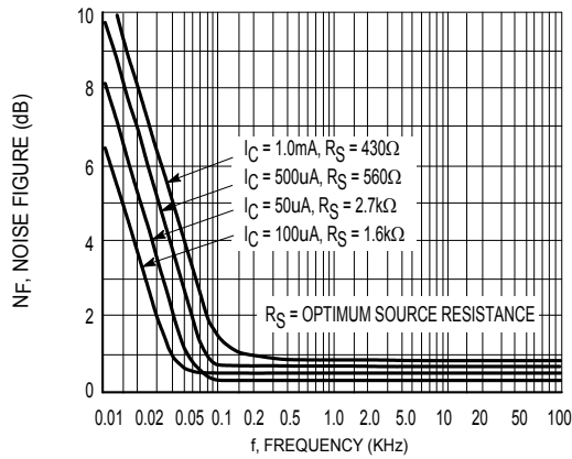
Figure 6. Frequency Effects
