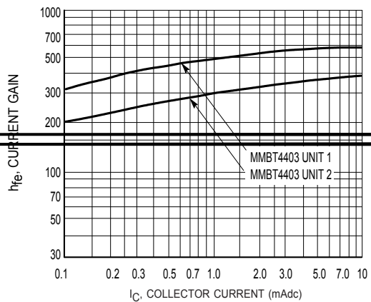
Figure 8. Current Gain
