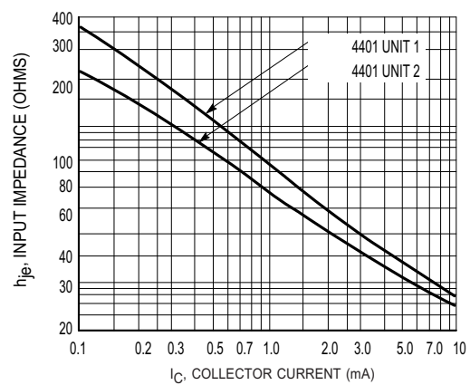
Figure 10. Input Impedance
