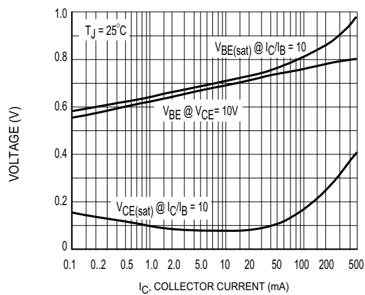
Figure 15. "ON" Voltages
