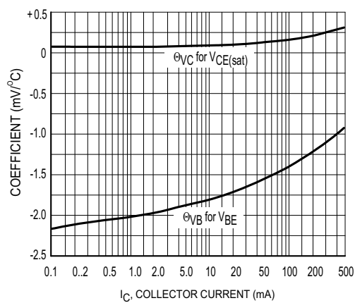
Figure 16. Temperature Coefficients
