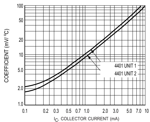
Figure 12. Temperature Coefficients
