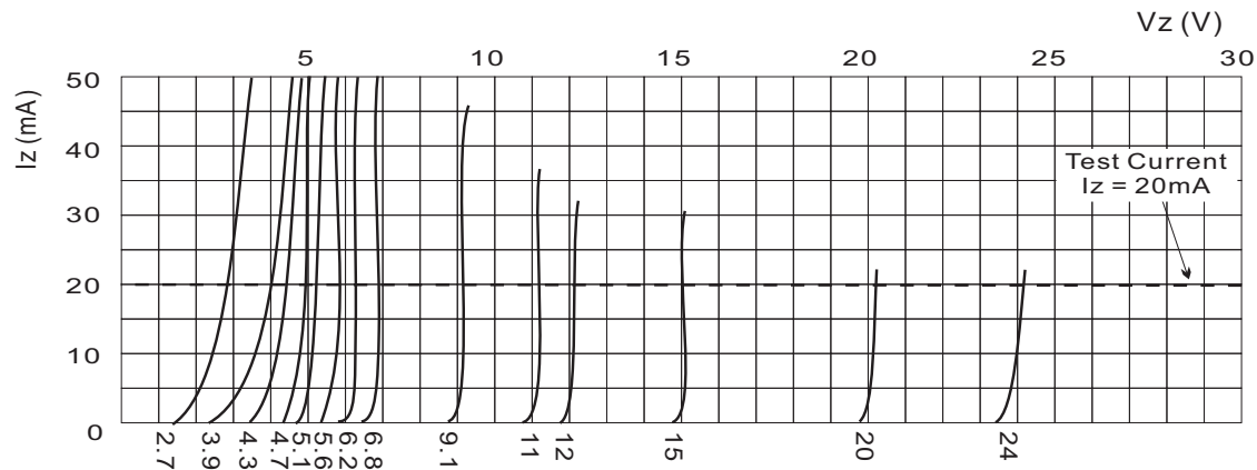
Fig.2 BREAKDOWN CHARACTERISTICS
