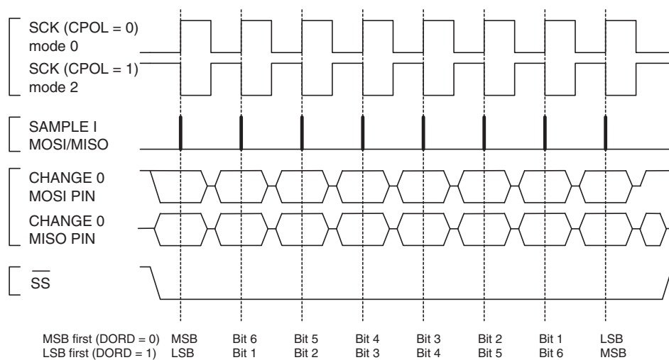
Figure 19-3. SPI Transfer Format with CPHA = 0
