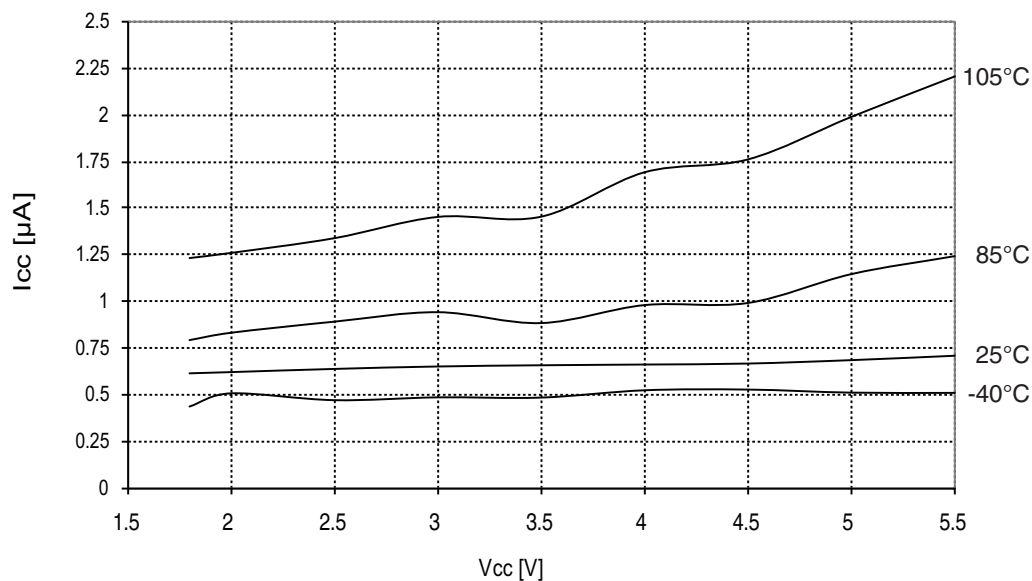
Figure 31-60. ATmega48PA: Power-Save Supply Current vs. V_{CC} (Watchdog Timer Disabled and 32kHz Crystal Oscillator Running)
