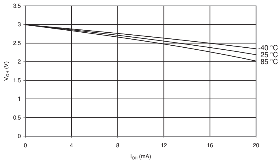
Figure 31-212. ATmega168A: I/O Pin Output Voltage vs. Source Current ( V_{CC} = 3\text{ V} )
