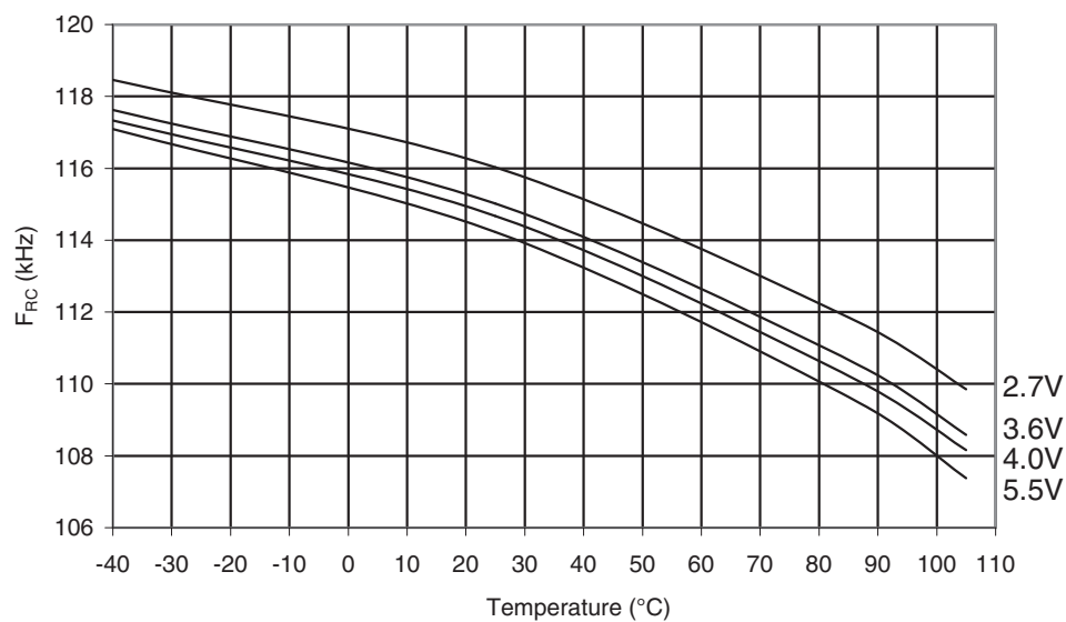
Figure 35-35. ATmega328P: Watchdog Oscillator Frequency vs. Temperature
