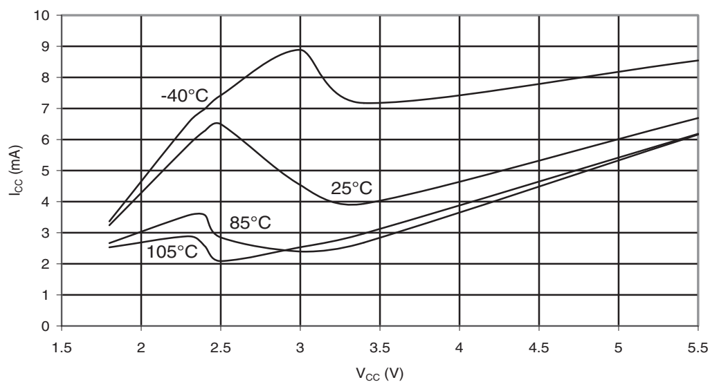
Figure 31-186. ATmega88PA: Programming Current vs. V_{CC}
