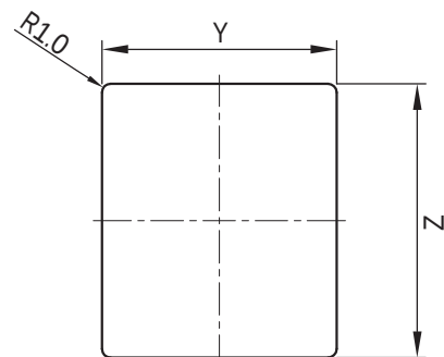
PANEL CUTOUT
