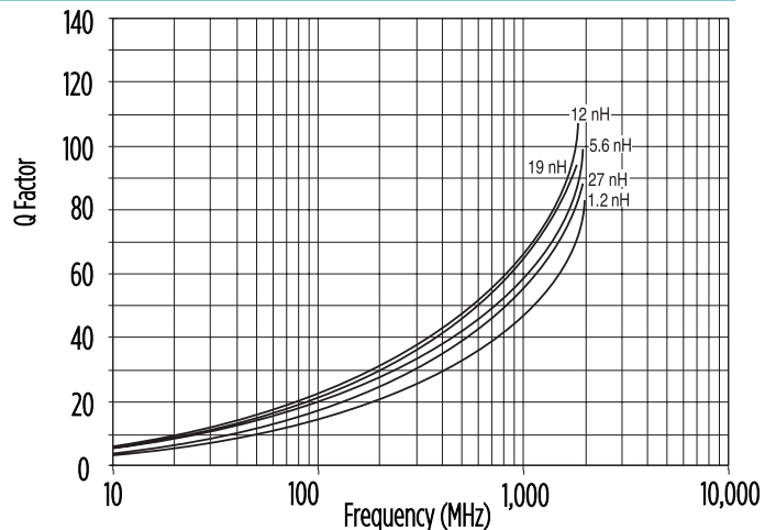
Typical Q vs Frequency
