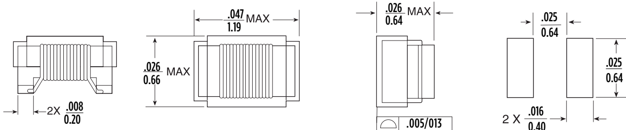
SUGGESTED PAD LAYOUT
