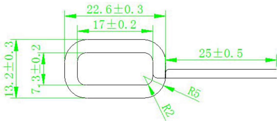
Coil
