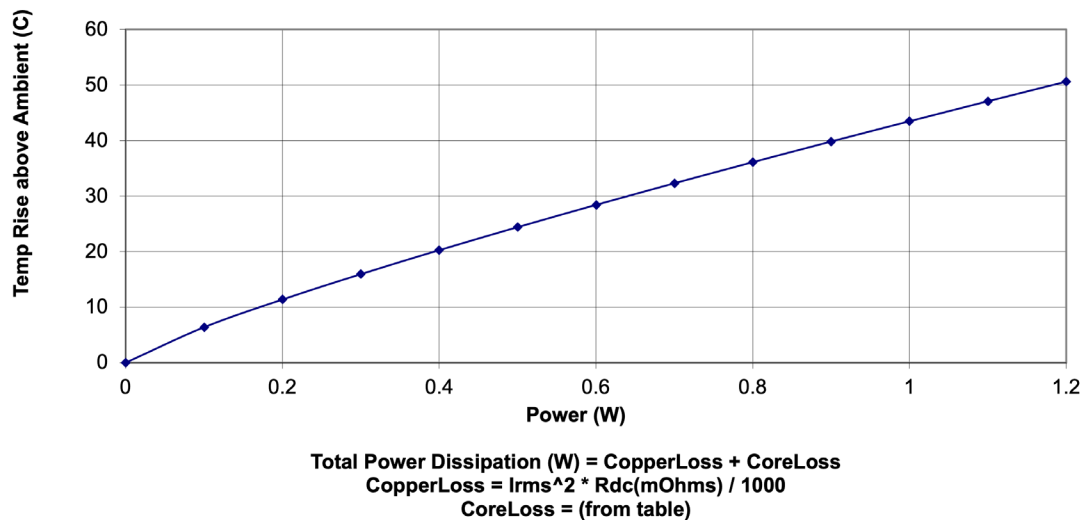
PA5034.XXXHLT Temp Rise vs Power Dissipation
