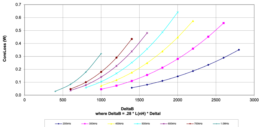
PA5034.XXXHLT CoreLoss (W)
