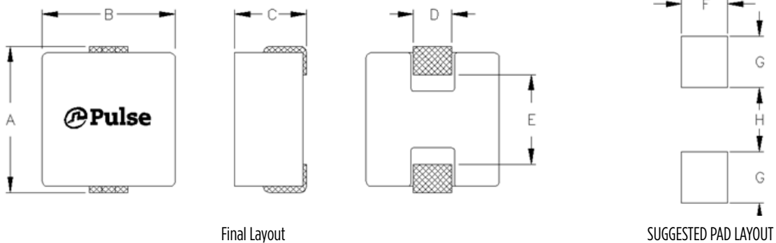
Final Layout
