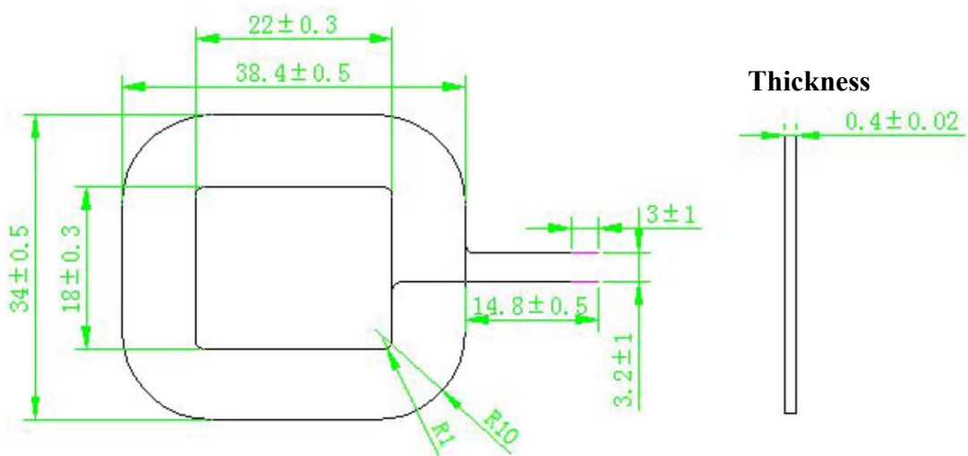
Coil
