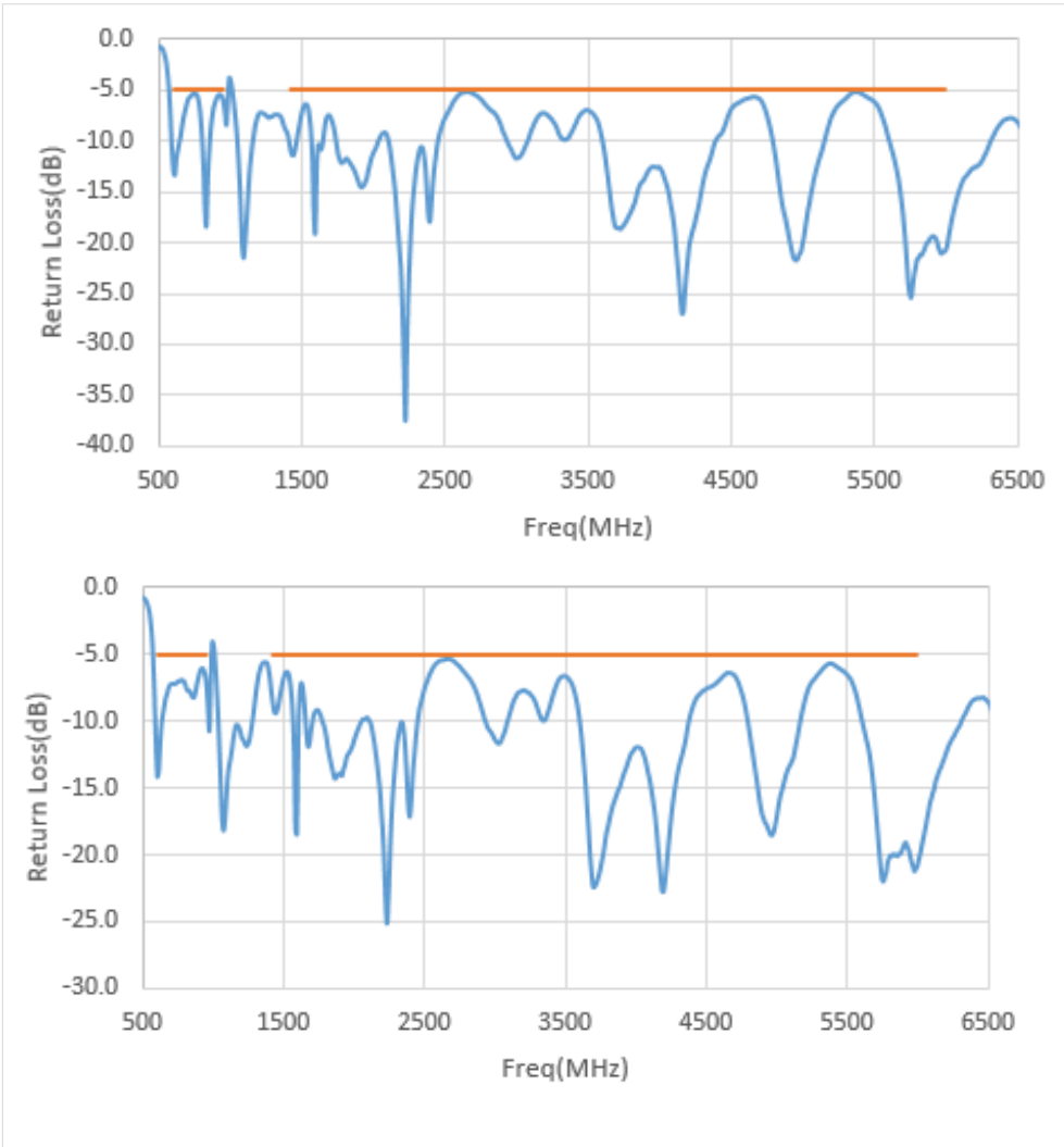
Return Loss
