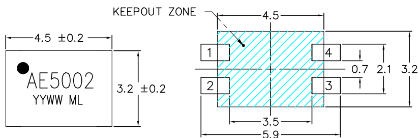
RECOMMENDED FOOTPRINT
