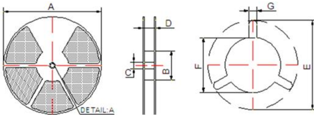
DETAIL A
