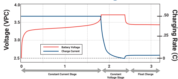
CHARGING CHARACTERISTICS @ C/2 AND 25°C
