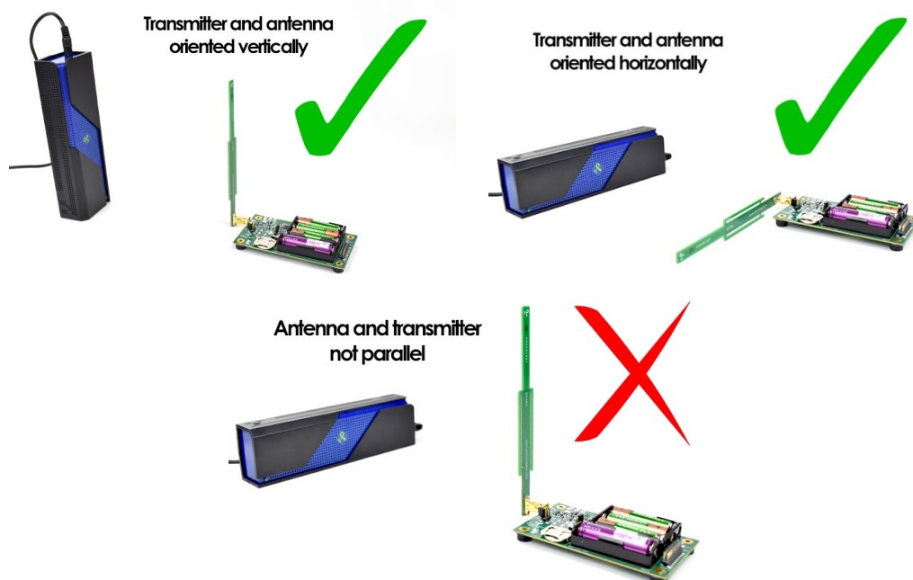
Fig. 4 – Correct Antenna Orientation
