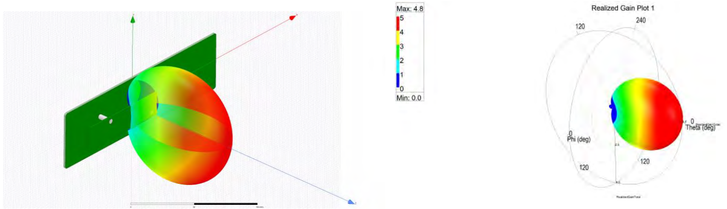
Radiation Pattern
