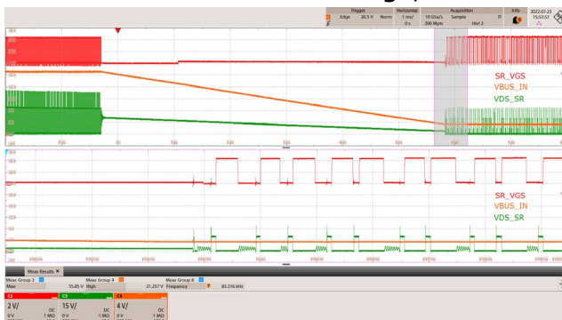
Figure 63 – SR FET Drain Voltage and Gate Voltage 90 VAC, 21 V to 3.3 V V_{OUT} Transition, 2.85 A Load.
