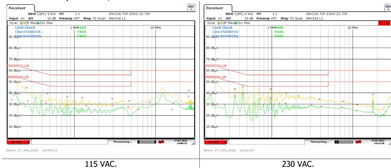
Figure 103 – Floating Ground EMI, 20 V / 3.25 A Load [Line Scan].
