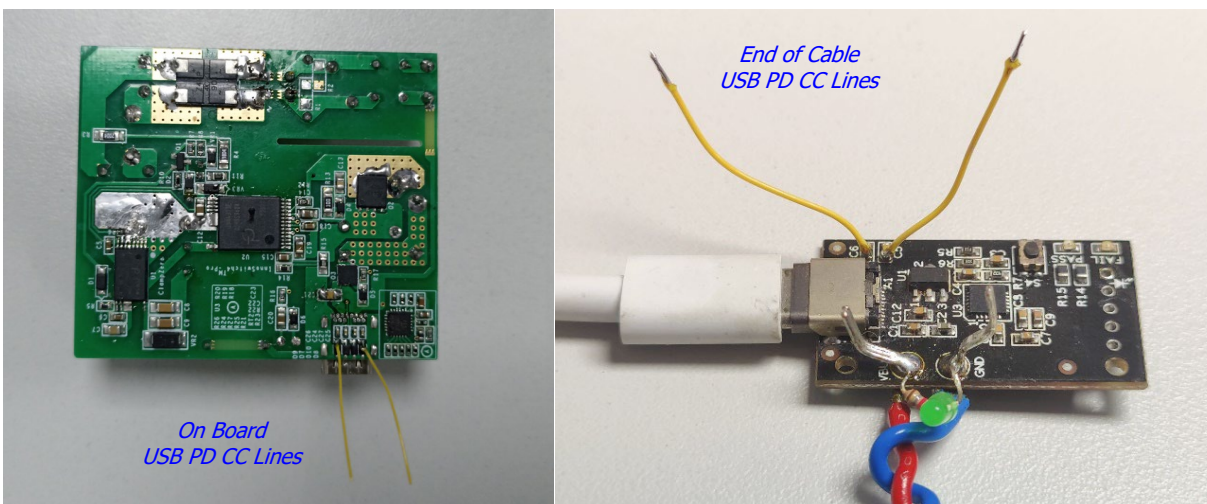
Figure 106 – ESD Discharge Points, USB PD Sink CC Lines.
