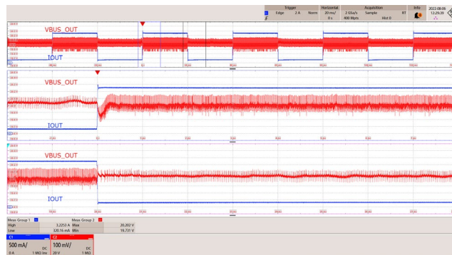
Figure 74 – Transient Response. 265 VAC, 20.0 V, 0.325 to 3.25 A Load. V_{BUS\_OUT} = 20.202 V Max., 19.731 V Min. CH1: I_{OUT} , 500 mA / div. CH2: V_{BUS\_OUT} , 100 mV / div. Time: 20 ms / div. (1 ms / div. Zoom).
