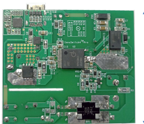
Figure 3 – Populated Circuit Board Photograph - Bottom.
