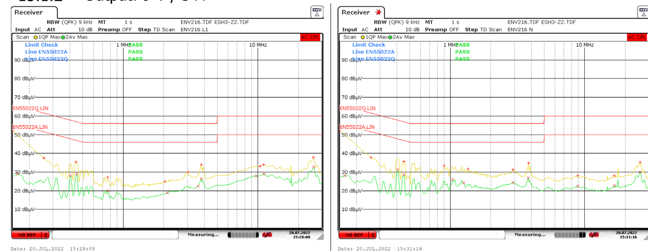
Figure 97 – Floating Ground EMI, 9 V / 3 A Load [Line Scan].
