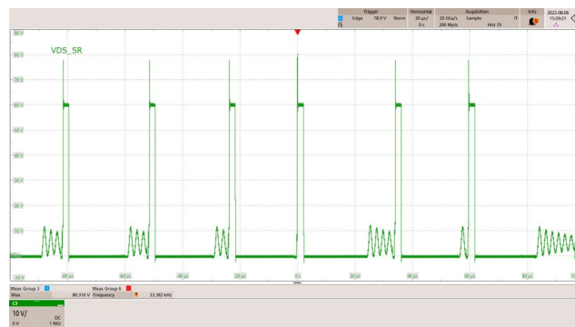
Figure 50 – SR FET Drain Voltage and Current. 265 VAC, 5.0 V, 3 A Load. V_{DS\_SR} = 80.316 V Maximum. CH1: V_{DS\_SR} , 10 V / div. Time: 20 μs / div.
