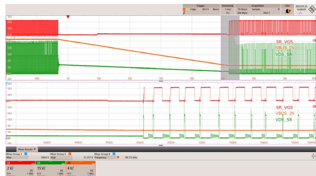
Figure 64 – SR FET Drain Voltage and Gate Voltage 265 VAC, 21 V to 5 V V_{OUT} Transition, 2.85 A Load.
