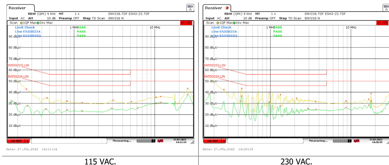
Figure 104 – Floating Ground EMI, 20 V / 3.25 A Load [Neutral Scan].
