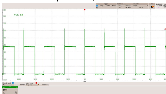
Figure 57 – SR FET Drain Voltage and Current. 90 VAC, 20.0 V, 3.25 A Load. V_{DS\_SR} = 62.925 V Maximum. CH1: V_{DS\_SR} , 10 V / div. Time: 10 μs / div.
