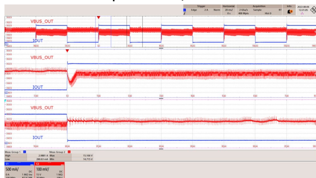
Figure 71 – Transient Response. 90 VAC, 15.0 V, 0.3 to 3 A Load. V_{BUS\_OUT} = 15.166 V Max., 14.715 V Min. CH1: I_{OUT} , 500 mA / div. CH2: V_{BUS\_OUT} , 100 mV / div. Time: 20 ms / div. (1 ms / div. Zoom).
