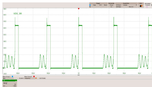
Figure 52 – SR FET Drain Voltage and Current. 265 VAC, 9.0 V, 3 A Load. V_{DS\_SR} = 76.364 V Maximum. CH1: V_{DS\_SR} , 10 V / div. Time: 10 μs / div.
