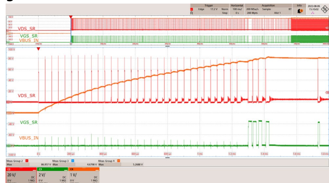
Figure 38 – SR FET Drain Voltage and Gate Voltage 265 VAC, 5.0 V, 3 A (CR Mode, 1.61 \Omega at the End of 100 m \Omega Cable). V_{DS\_SR} = 86.957 V Maximum. CH2: V_{DS\_SR} , 20 V / div. CH3: V_{GS\_SR} , 2 V / div. CH4: V_{BUS\_IN} , 1 V / div. Time: 100 ms / div. (200 \mu s / div. Zoom).
