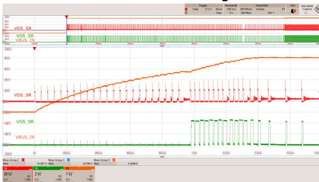
Figure 37 – SR FET Drain Voltage and Gate Voltage 90 VAC, 5.0 V, 3 A (CR Mode, 1.61 \Omega at the End of 100 m \Omega Cable). V_{DS\_SR} = 41.897 V Maximum. CH2: V_{DS\_SR} , 20 V / div. CH3: V_{GS\_SR} , 2 V / div. CH4: V_{BUS\_IN} , 1 V / div. Time: 100 ms / div. (200 \mu s / div. Zoom).
