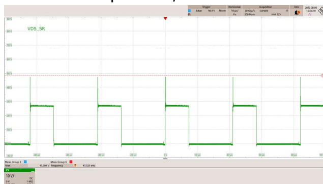
Figure 51 – SR FET Drain Voltage and Current. 90 VAC, 9.0 V, 3 A Load. V_{DS\_SR} = 47.508 V Maximum. CH1: V_{DS\_SR} , 10 V / div. Time: 10 μs / div.
