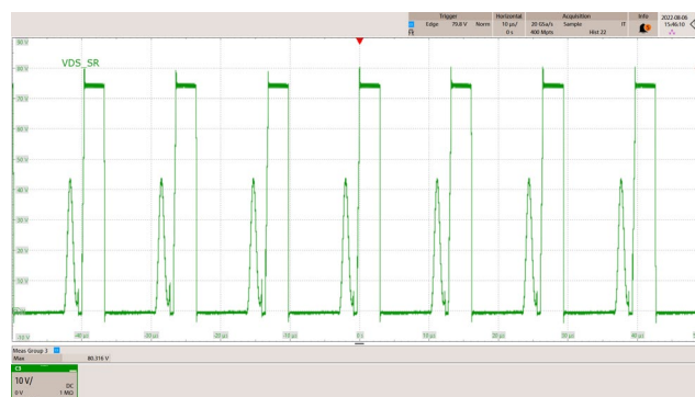
Figure 58 – SR FET Drain Voltage and Current. 265 VAC, 20.0 V, 3.25 A Load. V_{DS\_SR} = 80.316 V Maximum. CH1: V_{DS\_SR} , 10 V / div. Time: 10 μs / div.
