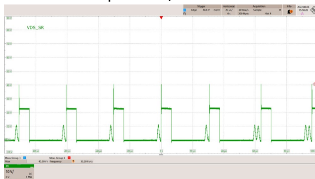
Figure 49 – SR FET Drain Voltage and Current. 90 VAC, 5.0 V, 3 A Load. V_{DS\_SR} = 40.395 V Maximum. CH1: V_{DS\_SR} , 10 V / div. Time: 20 μs / div.
