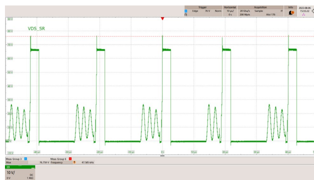
Figure 54 – SR FET Drain Voltage and Current. 265 VAC, 12.0 V, 3 A Load. V_{DS\_SR} = 76.759 V Maximum. CH1: V_{DS\_SR} , 10 V / div. Time: 10 \mu s / div.
