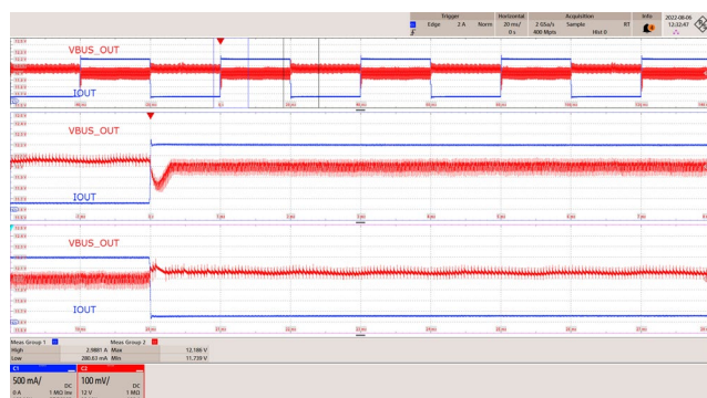
Figure 69 – Transient Response. 90 VAC, 12.0 V, 0.3 to 3 A Load. V_{BUS\_OUT} = 12.186 V Max., 11.739 V Min. CH1: I_{OUT} , 500 mA / div. CH2: V_{BUS\_OUT} , 100 mV / div. Time: 20 ms / div. (1 ms / div. Zoom).
