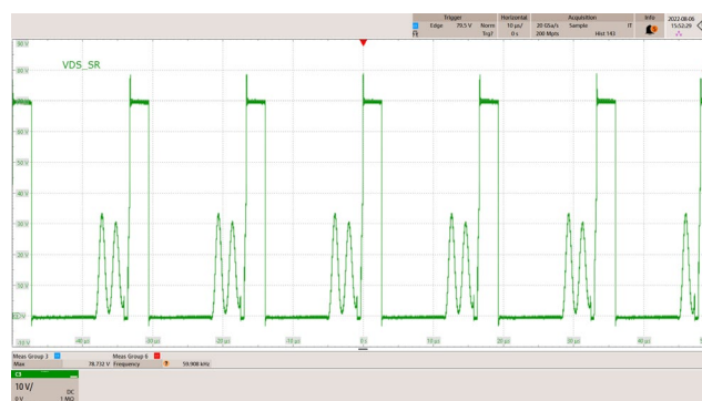
Figure 56 – SR FET Drain Voltage and Current. 265 VAC, 15 V, 3 A Load. V_{DS\_SR} = 78.732 V Maximum. CH1: V_{DS\_SR} , 10 V / div. Time: 10 \mu s / div.
