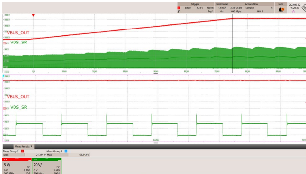
Figure 61 – SR FET Drain Voltage 90 VAC, 3.3 V to 21 V V_{OUT} Transition, 2.85A Load.
