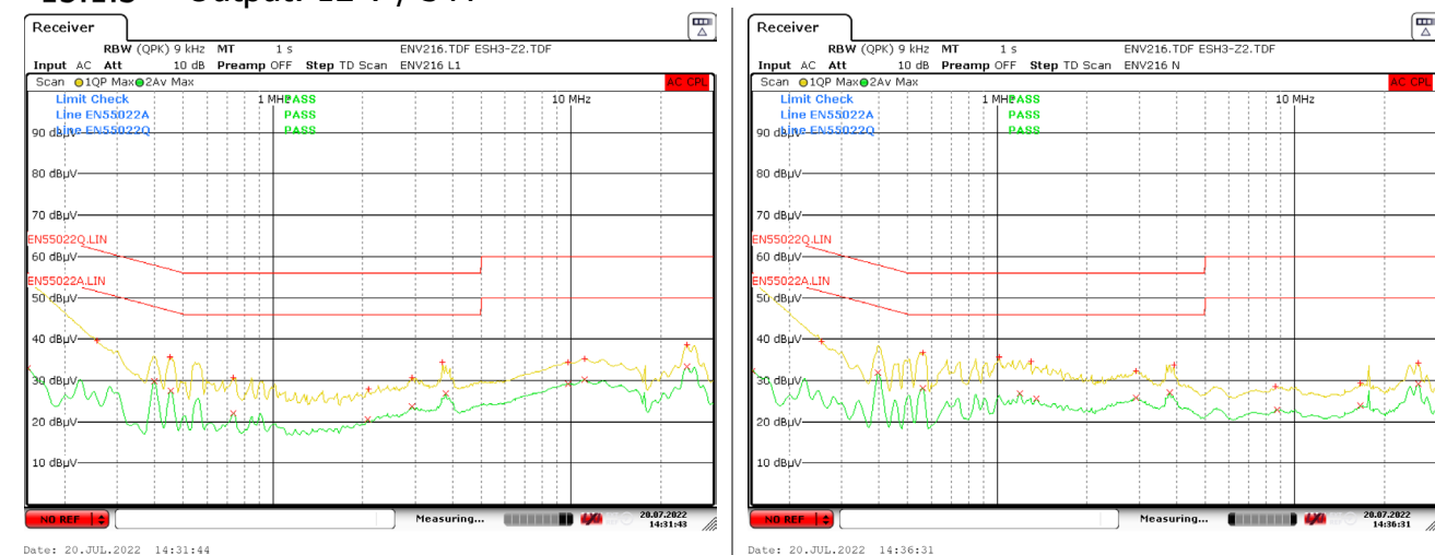
Figure 99 – Floating Ground EMI, 12 V / 3 A Load [Line Scan].
