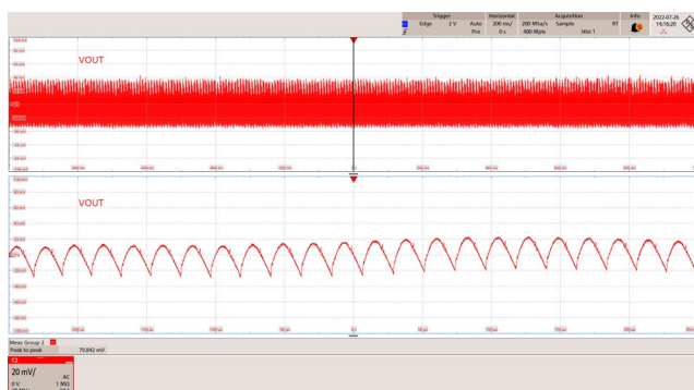
Figure 79 – Output Voltage Ripple. 90 VAC, 9.0 V, 3 A Load. V_{OUT(AC)} = 79.8 mV Peak-to-Peak. CH1: V_{OUT(AC)} , 20 mV / div. Time: 200 ms / div. (50 \mu s / div. Zoom).
