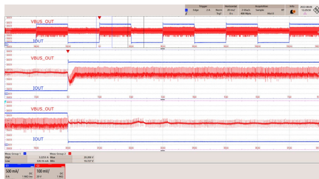
Figure 73 – Transient Response. 90 VAC, 20.0 V, 0.325 to 3.25 A Load. V_{BUS\_OUT} = 20.206 V Max., 19.727 V Min. CH1: I_{OUT} , 500 mA / div. CH2: V_{BUS\_OUT} , 100 mV / div. Time: 20 ms / div. (1 ms / div. Zoom).
