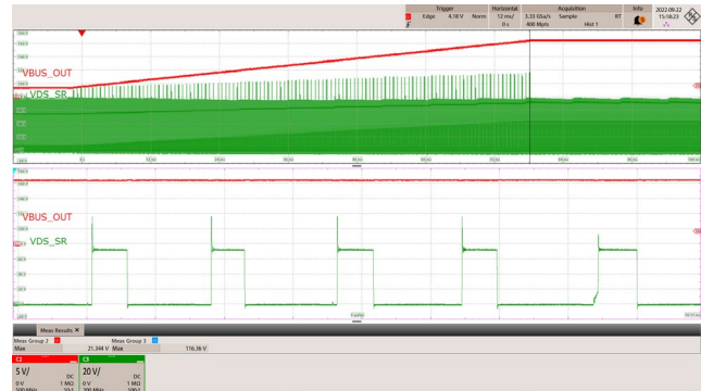
Figure 62 – SR FET Drain Voltage 265 VAC, 3.3 V to 21 V V_{OUT} Transition, 2.85 A Load.
