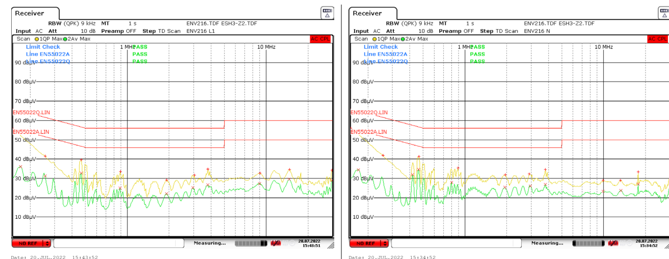
Figure 98 – Floating Ground EMI, 9 V / 3 A Load [Neutral Scan].
