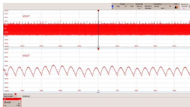
Figure 80 – Output Voltage Ripple. 265 VAC, 9.0 V, 3 A Load. V_{OUT(AC)} = 83 mV Peak-to-Peak. CH1: V_{OUT(AC)} , 20 mV / div. Time: 200 ms / div. (50 \mu s / div. Zoom).
