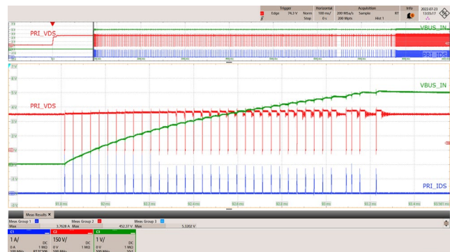
Figure 36 – Primary Drain Voltage and Current. 265 VAC, 5.0 V, 3 A (E-load CR Mode, 1.63 \Omega at the End of 100 m \Omega Cable). V_{DS\_PRI} = 452.37 V Maximum. CH1: I_{DS\_PRI} , 1 A / div. CH2: V_{DS\_PRI} , 150 V / div. CH3: V_{BUS\_IN} , 1 V / div. Time: 100 ms / div. (200 \mu s / div. Zoom).
