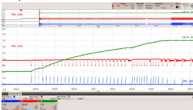
Figure 35 – Primary Drain Voltage and Current. 90 VAC, 5.0 V, 3 A (E-load CR Mode, 1.63 \Omega at the End of 100 m \Omega Cable). V_{DS\_PRI} = 197.43 V Maximum. CH1: I_{DS\_PRI} , 1 A / div. CH2: V_{DS\_PRI} , 150 V / div. CH3: V_{BUS\_IN} , 1 V / div. Time: 100 ms / div. (200 \mu s / div. Zoom).
